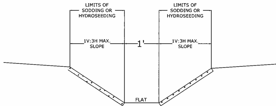
TYPICAL DITCH SECTION
